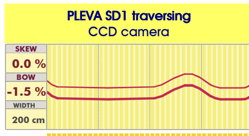
Distortion analysis based on 40 measuring points on 2000 mm fabric width
